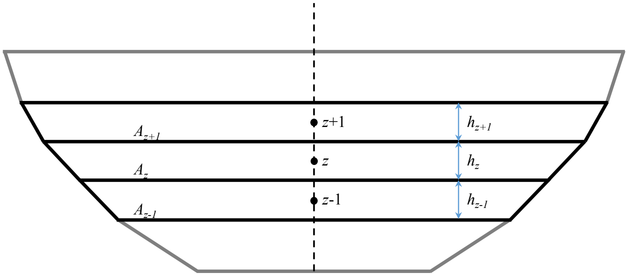
Fig. 5: Schematic of the staggered grid discretization of the lake medium used in the present study.
