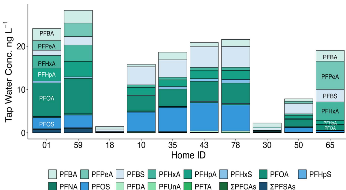
Fig. 2 PFAA profiles and concentrations in kitchen tap water samples. Compounds with DF > 50% are shown while those with DF < 50% were summed into their respective subclass (i.e., ΣPFCA or ΣPFSA). All carboxylic acids (PFCA) are in shades of green and the sulfonic acids (PFSA) are in shades of blue. Each bar is plotted such that PFBA is on top, followed by PFPeA and PFBS, with ΣPFCA and ΣPFSA last. Concentrations are mean field blank subtracted and corrected for recoveries.
