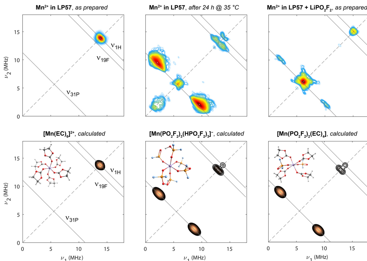
Fig. 2 Experimental (upper row) and calculated (lower row) HYSCORE spectra at 9.8 GHz (X-band; 20 K). Spectra from samples containing 8 mM Mn(TFSI) 2 dissolved in 1 M LiPF 6 in 3:7 EC:EMC (left), with mild heat-treatment at 35 °C for 24 h (centre), and addition of 80 mM LiPO 2 F 2 (right) are shown. Experiments were conducted at the magnetic field positions indicated by green arrows in Fig. 1. The diagonal is shown with a dashed line. Anti-diagonal (solid) lines are shown at relevant nuclear Larmor frequencies. Calculations are shown for three clusters, [Mn(EC) 6 ] 2+ , [Mn(PO 2 F 2 ) 3 (HPO 2 F 2 ) 3 ] - and [Mn(PO 2 F 2 ) 2 (EC) 4 ].
