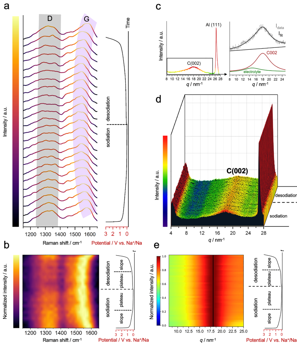
Fig. 3 (a) Raman spectra of the HC during sodiation and desodiation, revealing slight intensity q changes in the D-band and a sharp shift in the G-band. (b) A heat map with normalized intensity visualizes the pronounced shift in the G-band during sodiation and desodiation. (c) Operando WAXS pattern, showing the C(002) peak of hard carbon alongside contributions from the Al current collector and a broad, insignificant background from the electrolyte. The C(002) peak is resolved and isolated via peak fitting, with no overlap from electrolyte contributions. (d) WAXS patterns during sodiation and desodiation, revealing no shift in the C(002) but a slight decrease in intensity at the beginning of the electrochemical process. (e) Normalized heat map of the deconvoluted C(002) peak visualizes no pronounced shift during the electrochemical processes.
