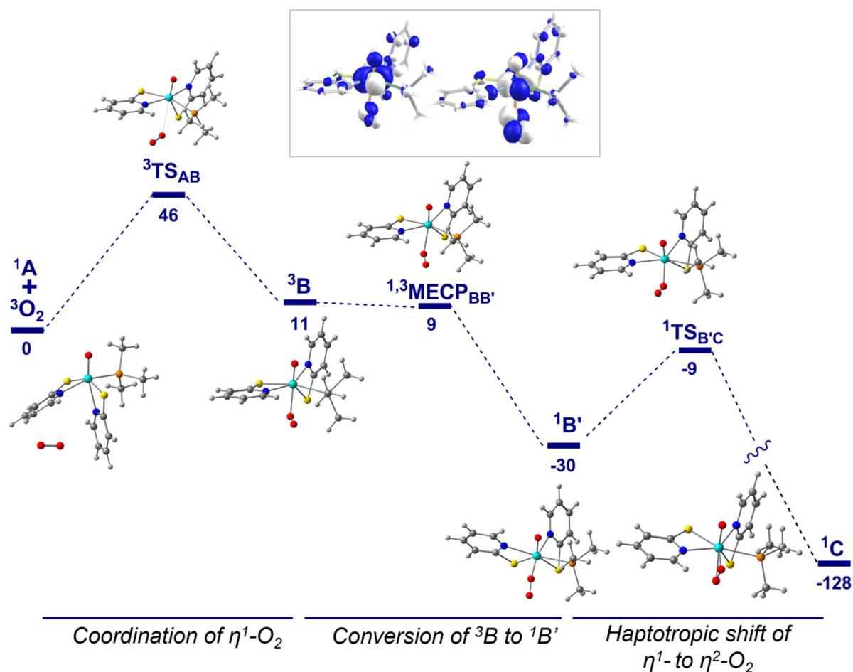
Fig. 2 Dioxygen activation: the interaction of ^3\text{O}_2 with ^1[\text{W}(\text{IV})\text{O}(\text{PyS})_2(\text{PMe}_3)] (A) and the quasi-restricted single occupied orbitals (SOMOs in the inlet) of the complex at the triplet state of ^{1,3}\text{MECP}_{\text{BB}'} (energies in \text{kJ mol}^{-1} ).
