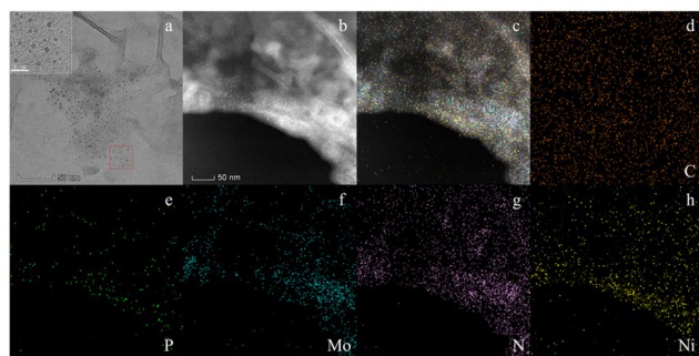
Fig. 1 (a–b) TEM of Ni-P 4 Mo 6 /GO. (c–h) Element mapping of images of Ni-P 4 Mo 6 /GO.
