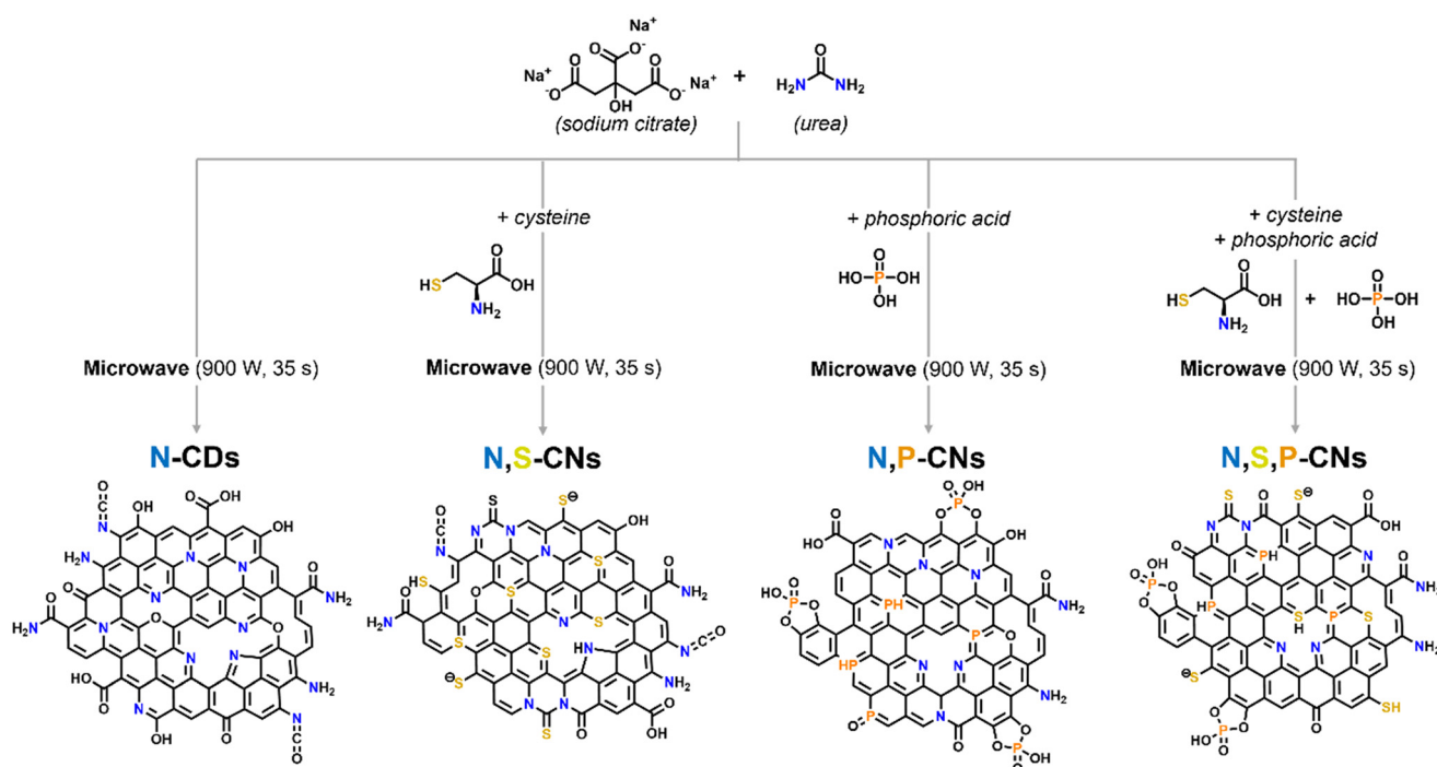
Scheme 1 Methodology for the synthesis of the multi-doped carbon nanomaterials: N-CDs; N,S-CNs; N,P-CN; and N,S,P-CN.
