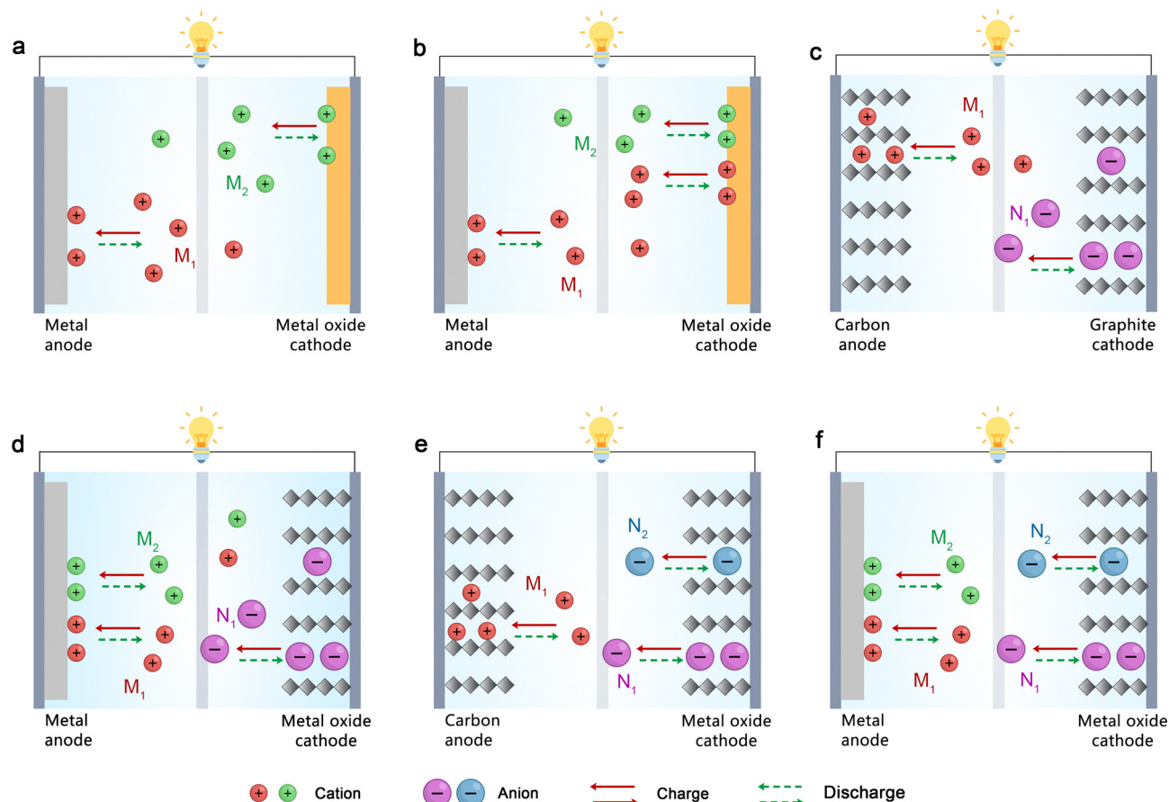
Fig. 2 Schematic illustration of representative hybrid battery configurations based on different charge carrier types: (a) and (b) dual-cation systems; (c) cation–anion dual-ion system; (d) triple-ion system with two cations and one anion; (e) triple-ion system with one cation and two anions; and (f) quadruple-ion system comprising two cations and two anions.
