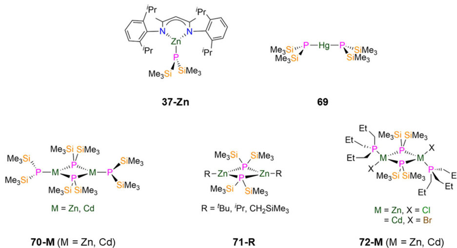
Fig. 20 Monomeric and dimeric group 12 P'' complexes [Zn(\text{DippNacnac})(P'')] ( 37-Zn ; \text{DippNacnac} = \text{CH}\{(\text{CH}_3)_2\text{CN}(\text{Dipp})\}_2 ; \text{Dipp} = \text{C}_6\text{H}_3\text{Pr}_{2-2,6} ), [\text{Hg}(P'')]_2 ( 69 ), [M(P'')(\mu-P'')]_2 ( 70-M , M = Zn, Cd ), [Zn(R)(\mu-P'')]_2 ( 71-R , R = ^t\text{Bu}, ^i\text{Pr}, \text{CH}_2\text{SiMe}_3 ), [M(P''\text{Pr}_3)(X)(\mu-P'')]_2 ( 72-Zn : M = Zn , X = \text{Cl} ; 72-Cd : M = Cd , X = \text{Br} ).
