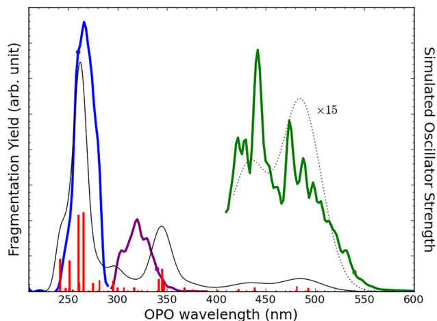
Fig. 3 Optical action (fragmentation) spectrum of [\text{Mo}_6\text{I}_{14}]^{2-} in the UV-visible range. The photo-fragmentation was recorded independently for three regions: < 290\text{ nm} (blue), [290-390]\text{ nm} (purple) and > 410\text{ nm} (green). Laser irradiance and alignment conditions vary between regions so that their absolute intensities should not be compared. Thus, experimental data was scaled to ease the comparison with the simulated spectrum. Data were recorded with a 2\text{ nm} pitch. Circles on the experimental curves represent the position of the laser alignment for each spectral range. The simulated spectrum (thin black line) is calculated from 0.12\text{ eV} Gaussian convolution of the oscillator strength for each transition (red bars). A factor \times 15 is applied to simulated data in the visible range (dotted line).
