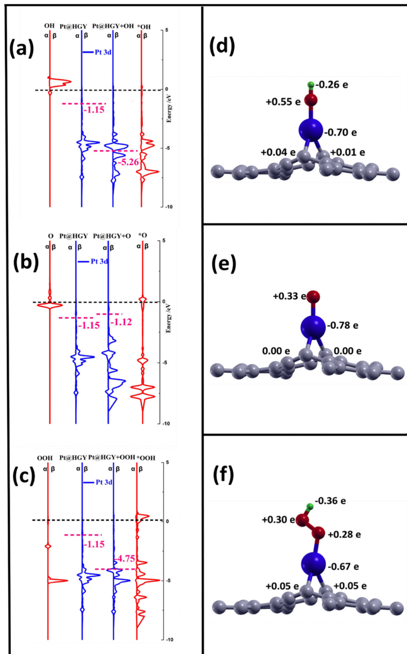
Fig. 7 (a)–(c) PDOS and diagrammatic representation of 3d orbitals of Pt@HGY, where the solid blue line embodies the Pt 3d orbitals. 2p orbitals of intermediates prior and subsequent to the adsorption on the Pt@HGY substrate. The pink dotted line marks the position of the d band centre of the Pt@HGY substrate prior and subsequent to the adsorption of O, OH, and OOH. Lőwdin charge analysis (d)–(f) of the corresponding adsorbed OH, O, and OOH. Colour scheme: silver C; navy blue Pt; green H; red O.
