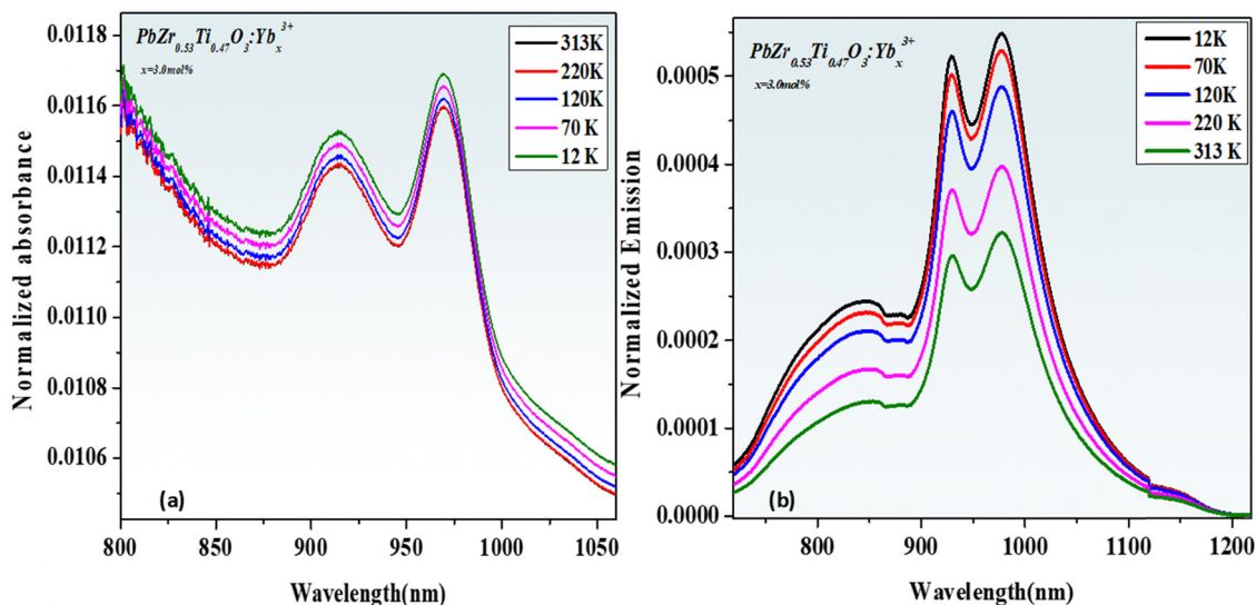
Fig. 10 Normalized (a) absorption and (b) emission spectra of the Yb 3+ :PZT host at different temperatures.
