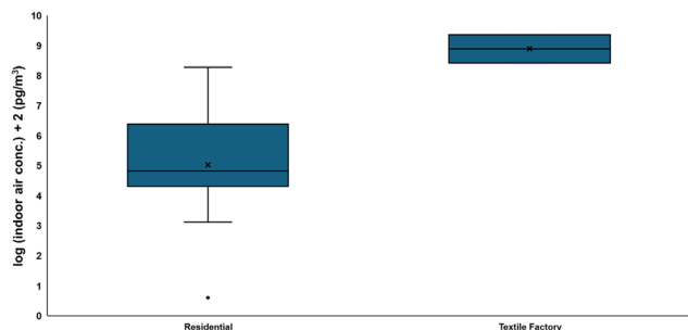
Levels of FTOHs released to air collected near industrial sites, namely near textile and carpet manufacturing and treatment, 77,102,201,240 and fluorochemical manufacturing facilities, 241,242 are two-to-three orders of magnitude and one order of magnitude higher than the levels of FTOHs collected near non-industrial sites, 70,75,79–83,86–88,91,93,96,113,114,117,121,207,211,212,243–266 respectively (Fig. 4). Of note, FTOH release from textile and carpet manufacturing and treatment facilities can be one-to-two
