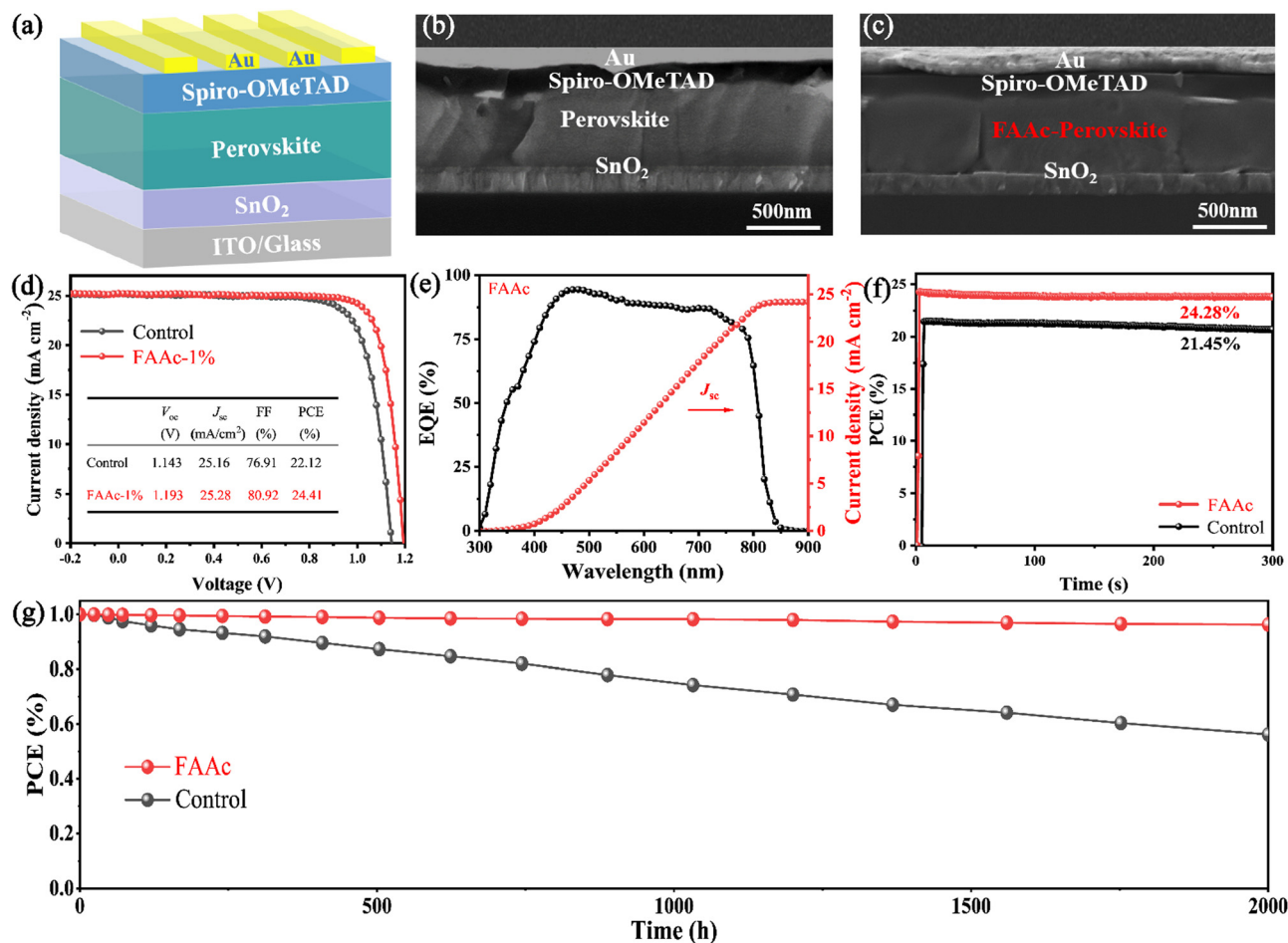
Fig. 5 (a) The schematic diagram of the device structure. Cross-sectional SEM image of the (b) control and (c) FAAC-modified perovskite device structures. (d) J-V curves of the control and FAAC-modified PSCs. (e) EQE and the integrated J_{sc} of FAAC-PSCs. (f) Steady-state PCE at the maximum power point for the control and FAAC-modified PSCs. (g) Stability test of devices.
