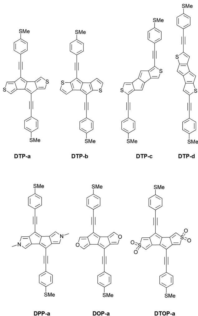
Fig. 1 Lewis structures of a selection of compounds investigated in this study. Top panel: Isomers of dithienopentalene (DTP). Bottom panel: Isomer a for di- N -methylpyrrolopentalene (DPP), di-furylpentalene (DOP) and di-thiophene- S,S -dioxide (DTOP); isomers b , c and d for each heteroatom have the same anchor group position as in the respective DTP isomers above.
