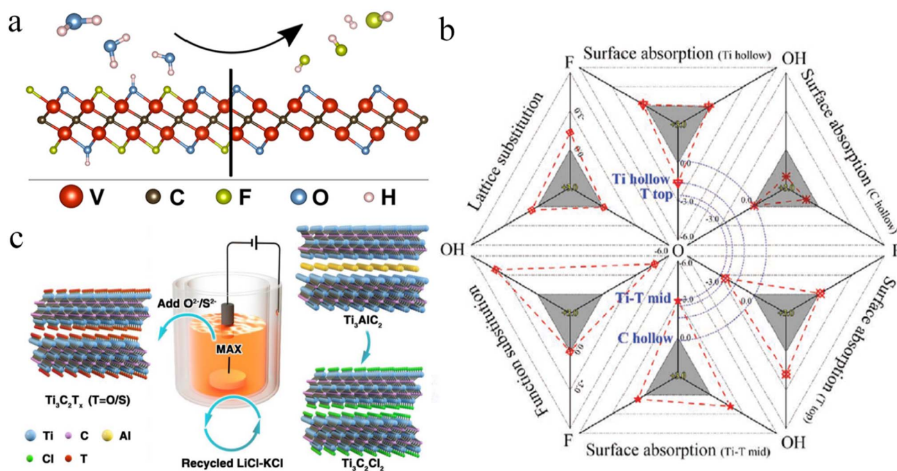
Fig. 8 (a) Removal of fluoride terminations by gas hydrolysis, reproduced from ref. 147 with permission from American Chemical Society, copyright 2022. (b) Simulation with nitrogen dopants in Ti 3 C 2 , reproduced from ref. 149 with permission from Wiley, copyright 2020. (c) MXene synthesis by molten salt etching, reproduced from ref. 151 with permission from Wiley, copyright 2021.
