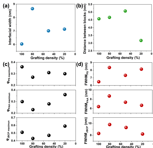
Fig. 6 Characteristics of segment density distributions for different grafting densities (GD) with N_{BB} = 100 . (a) Interfacial width solved from PS[(DPS-PAA) n ][DP2VP] Si . (b) Distance (d) between two blocks (c) volume fraction maximum ( \phi_{\text{maximum}} ) of PS block, PAA block and JBCP molecule. (d) Full-width half maximum (FWHM) of PS block, PAA block and JBCP molecule.
