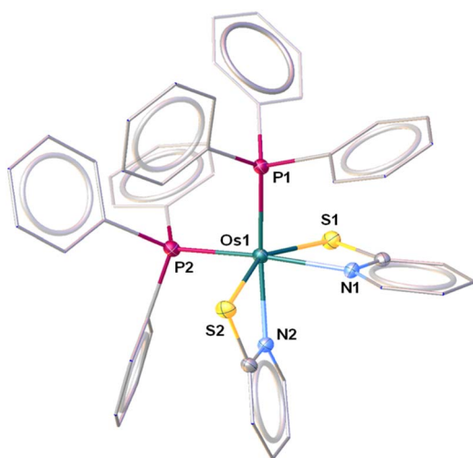
Fig. 1 Molecular structure and labelling diagram of 2b . Selected bond lengths (Å) and bond angles ( ^\circ ) of 2b : Os1–N1 2.143(3), Os1–N2 2.134(3), Os1–P1 2.2887(10), Os1–P2 2.2993(10), Os1–S1 2.4318(10), Os1–S2 2.4257(10); S2–Os1–S1 150.98(4), and N2–Os1–N1 80.11(13).
