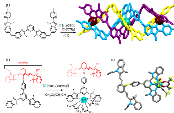
Fig. 6 (a) Heterotrinitopic ligand L1 used in the preparation of the heterotrinitopic [\text{Cr}_2\text{Er}(\text{L}1)_3]^{9+} complex displaying NIR to visible ETU UC. 29 (b) NIR dye containing tridentate ligand L2 displaying ligand to Er ETU UC. 72 with (c) single-crystal X-ray structure (ion colors: Cr = brown, Er = teal).
