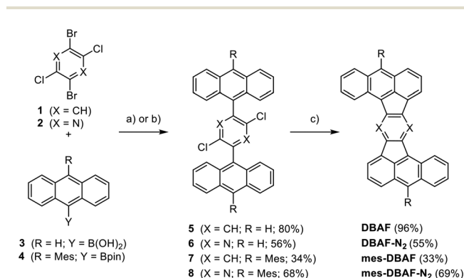
Scheme 1 Synthesis of DBAF, DBAF-N 2 , mes-DBAF and mes-DBAF-N 2 from dibromodichlorobenzene 1 and dibromodichloropyrazine 2 . (a) For 5 and 7 : Pd(OAc) 2 (2.5–3 mol%), SPhos (5–6 mol%), K 2 CO 3 (1 M), THF, 85 °C, 16 h; for 6 and 8 : (b) Pd(dppf)Cl 2 (10 mol%), K 2 CO 3 (1 M), THF, 85 °C, 16 h, (c) PdCl 2 (PCy 3 ) 2 , DBU, DMAc, 200 °C, 16 h.
