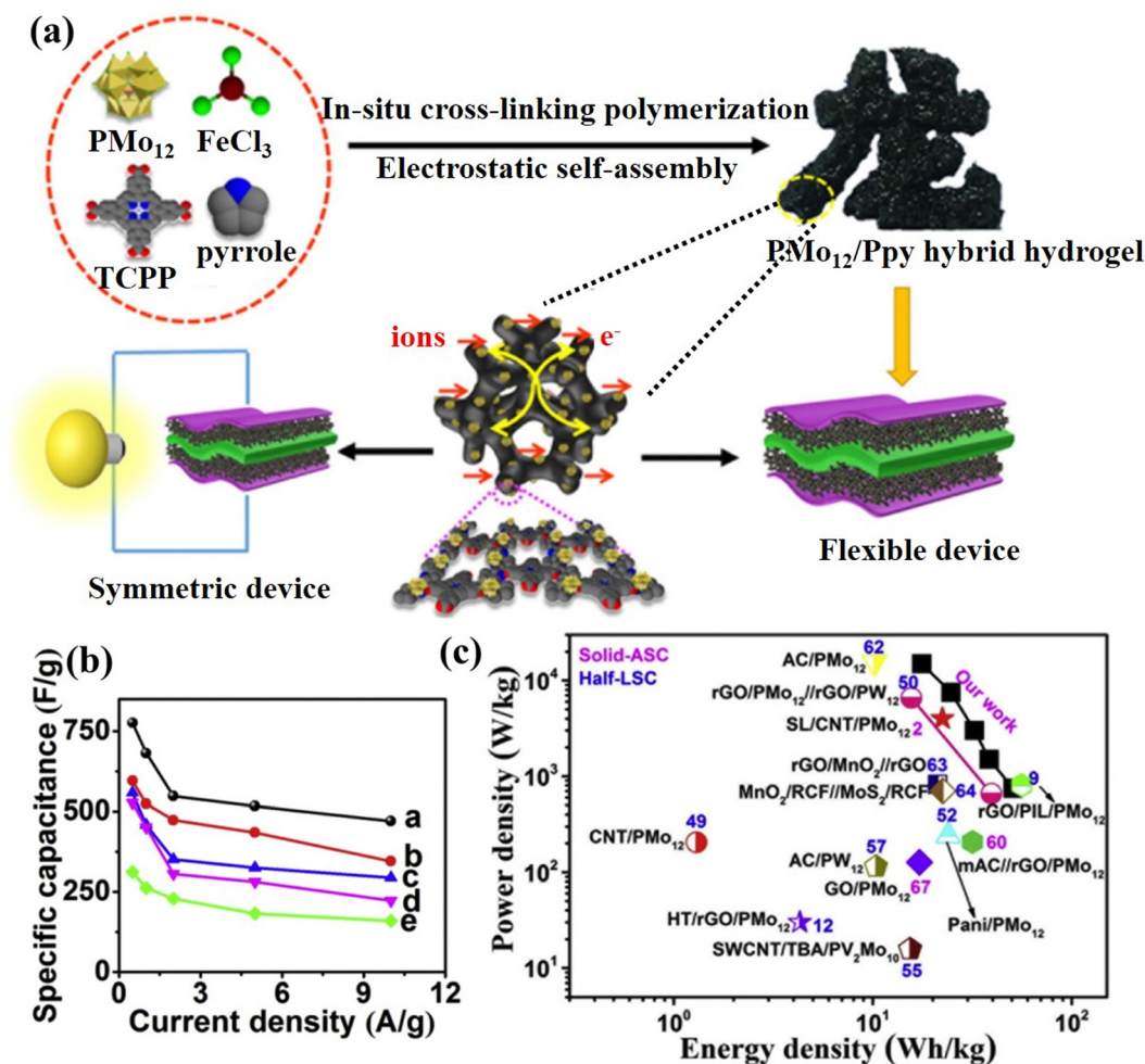
Fig. 22 (a) The preparation process for the PMo 12 /PPy hybrid hydrogel for SCs. (b) Specific capacitances of the prepared samples at various current densities. (c) Ragone plots of the P 2 -PPy gel//P 2 -PPy gel device compared with the values reported for other devices. 203 Copyright 2019, Elsevier Ltd.
