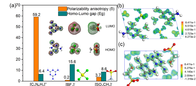
Fig. 10 (a) The polarizability anisotropy and HOMO–LUMO gap for the [C 3 N 6 H 7 ] + , [BF 4 ] - , [SO 3 CH 3 ] - groups. The EDD of MELBF (b) and MELSC (c).
