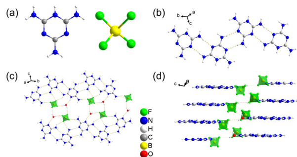
Fig. 2 Crystal structure of MELBF. (a) Basic constituent units [\text{C}_3\text{N}_6\text{H}_7]^+ and [\text{BF}_4]^- . (b) The one-dimensional chain formed by [\text{C}_3\text{N}_6\text{H}_7]^+ groups. (c) The two-dimensional structure formed by [\text{C}_3\text{N}_6\text{H}_7]^+ and [\text{BF}_4]^- groups. (d) Three-dimensional structure.
