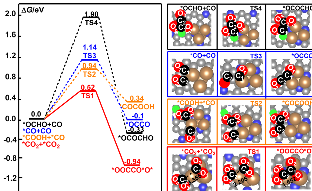
Fig. 3 The calculated free energy profiles for the direct coupling of two ^{\circ}\text{CO}_2 , ^{\circ}\text{OCHO} and \text{CO} , ^{\circ}\text{COOH} and ^{\circ}\text{CO} , and two \text{CO} molecules to form a C–C bond on the surface of the \text{Cu}_4/\text{N}_3\text{GN} catalyst.
