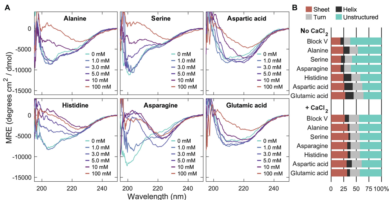
Fig. 5 Consensus repeat variants formed consistent calcium-bound structures. (A) All consensus repeat variants produced similar circular dichroism spectra at 100 mM CaCl 2 (red curves), which were characterized by a monotonic decrease from 200 nm to 220 nm and a broad negative peak near 225 nm. Replicate spectra of all consensus repeat variants are included in Fig. S22–S27.† (B) CD spectral deconvolution at 0 mM and 100 mM CaCl 2 revealed a structural variation among consensus repeat variants in the absence of calcium, in contrast to quantitatively similar structures in the presence of 100 mM CaCl 2 .
