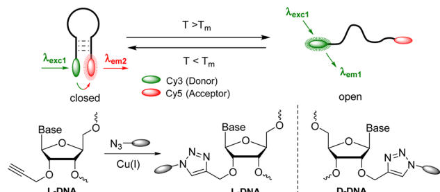
Fig. 1 Concept of wavelength-shifting molecular beacons made of L- or D-DNA, with an L- or D-configured clickable anchor for the chromophores.
