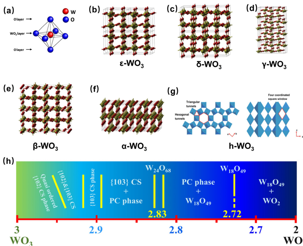
Fig. 2 (a) Ideal WO 3 crystal. (b) Monoclinic WO 3 . (c) Triclinic WO 3 . (d) Monoclinic WO 3 (17–330 °C). (e) Orthorhombic WO 3 . (f) Tetragonal WO 3 . (g) Hexagonal WO 3 . Reproduced with permission. 4 Copyright 2019, John Wiley and Sons. (h) Sub-stoichiometric WO 3-x . Reproduced with permission. 12 Copyright 2021, Springer Nature.
