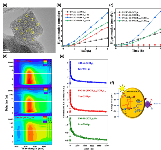
Fig. 3 (a) HRTEM image of \text{UiO-66}-(\text{SCH}_3)_2\text{-9h} deposited with Pt. Results of photocatalytic \text{H}_2 production under visible light illumination over (b) \text{Pt/UiO-66}-(\text{SCH}_3)_2 and \text{Pt/UiO-66}-(\text{SCH}_3)_2\text{-xh} , (c) \text{Pt/UiO-66}-(\text{SOCH}_3)_x(\text{SCH}_3)_{2-x} ( x = 0, 0.4, 0.6, 2 ). (d) TA spectra at various probe delays and wavelengths for \text{UiO-66}-(\text{SCH}_3)_2 , \text{UiO-66}-(\text{SOCH}_3)_{0.4}(\text{SCH}_3)_{1.6} , and \text{UiO-66}-(\text{SCH}_3)_2\text{-9h} . (e) Corresponding kinetic traces at 640 nm. The pump wavelength was 400 nm. (f) Proposed mechanism of interfacial charge transfer for \text{UiO-66}-(\text{SCH}_3)_2\text{-xh} . Reproduced with permission from ref. 40. Copyright 2021, American Chemical Society.
