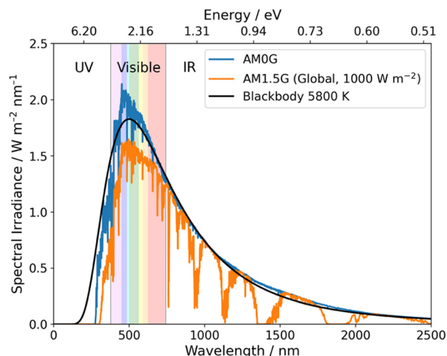
Fig. 2 Blackbody irradiance curve at 5800 K and standard solar spectra for space (AM0G) and terrestrial (AM1.5G). Data obtained from ref. 18.
