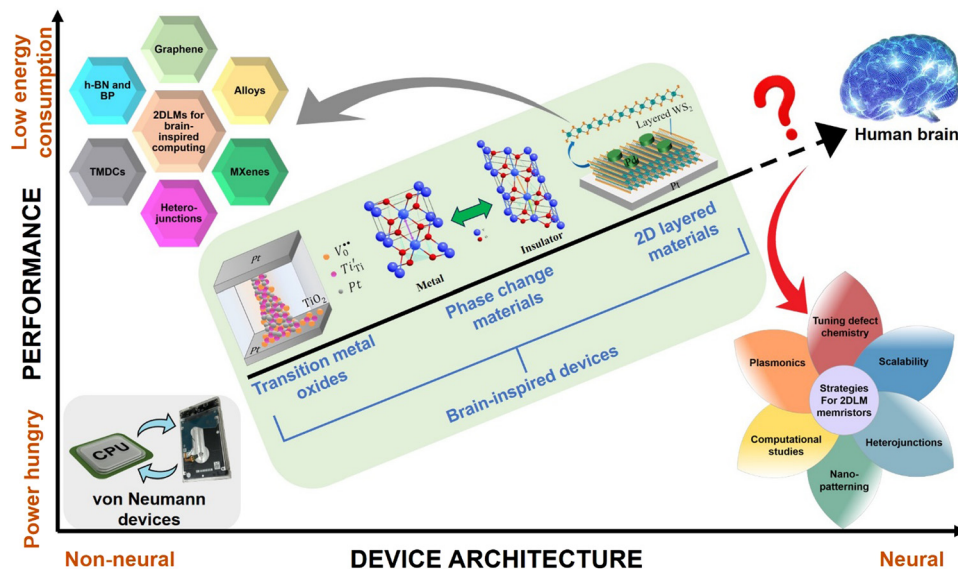
Fig. 6 2DLs for neuromorphic computing. Performance scales up with the advancement of the design architecture, ranging from von Neumann devices to neuromorphic systems. The ultimate target is to design devices mimicking brain's activity and matching its efficiency. Recent progress in memristors fabricated utilizing TMOs, PCMs, and 2DLs, and with certain strategic modifications in different 2DLs, devices emulating intelligence and critical for non-von Neumann machines can be designed. Reproduced with permission from ref. 87, 119 and 120. Copyright 2019, John Wiley & Sons, Inc.; copyright 2023, Springer Nature; copyright 2020, Frontiers.
