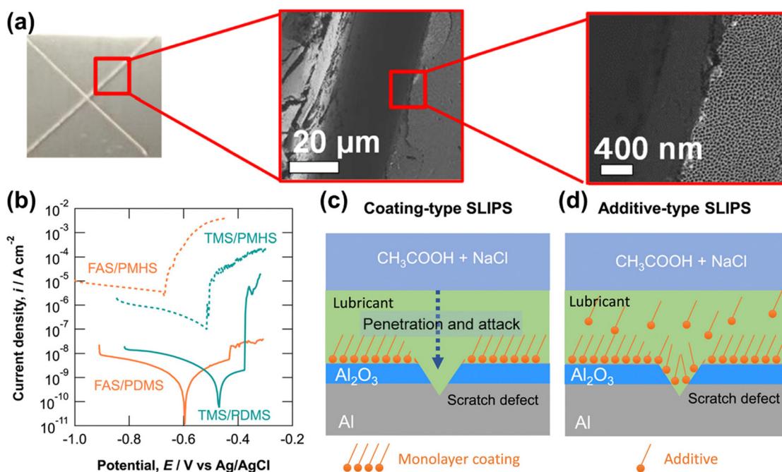
Fig. 19 Potentiodynamic polarization curves of the additive-type SLIPs measured after immersion in 2 g dm^{-3} acetic acid containing 10 g dm^{-3} NaCl (pH 3) for one week and subsequent introduction of the scratch defects, and schematic illustrations of coating-type and additive-type SLIPs with a scratch defect (reproduced from ref. 208 with permission from [American Chemical Society], copyright [2021]).
