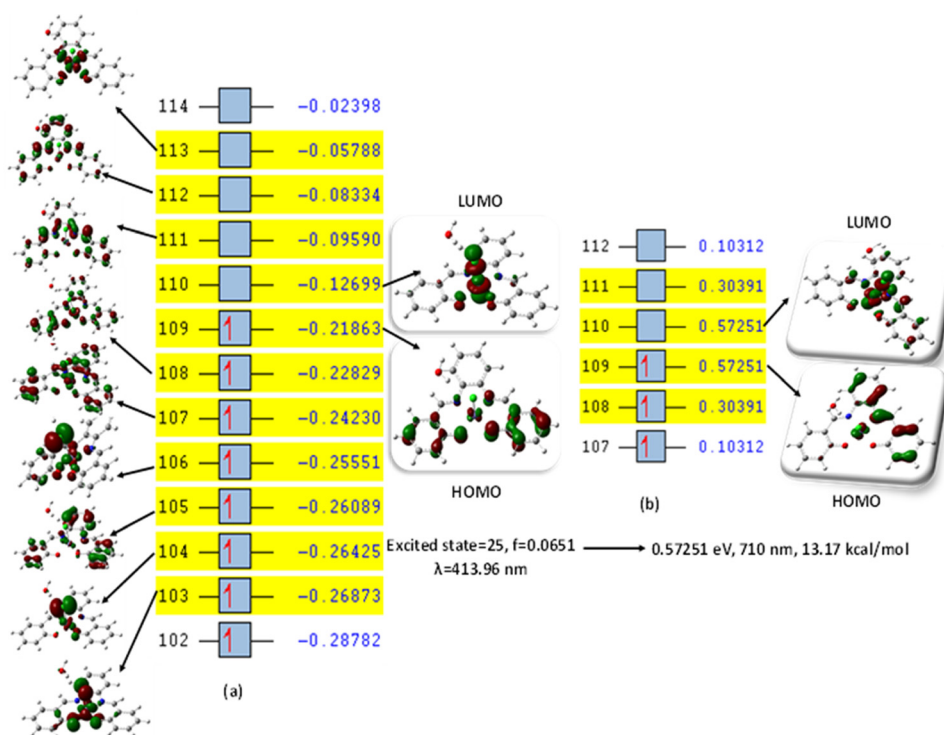
Fig. 9 (a) Canonical orbitals involved in the 16th excited state according to TD-DFT. (b) NTOs for [Fe(SALPHEN)Cl(H 2 O)]. Orbital 109 (particle) and orbital 110 (hole) exhibit the largest occupancies for excited state no. 25. [Fe(SALPHEN)Cl(H 2 O)] at a multiplicity of S = 1/2 , determined with B3LYP/DGDZVP.
