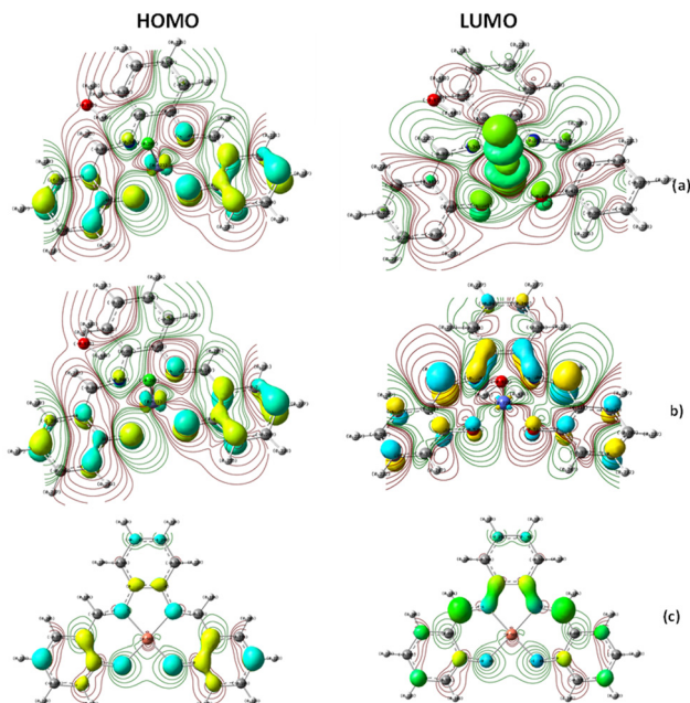
Fig. 14 Electron density isosurface (contour 0.05 \text{ e } \text{Å}^{-3} ), HOMO, and LUMO derived at the B3LYP/DGDZVP level. HOMO and LUMO contour plots (isosurface value = 0.05 \text{ a.u.} ) of the complexes: (a) [\text{Fe}(\text{SALPHEN})\text{Cl}(\text{H}_2\text{O})] , (b) [\text{Co}(\text{SALPHEN})(\text{H}_2\text{O})] , and (c) [\text{Cu}(\text{SALPHEN})] in the gaseous state. Color code used for the structure of molecules: C (grey), H (white), N (blue), O (red) and metal ions (turquoise/blue for \text{Fe}(\text{III}) and \text{Co}(\text{II}) ; turquoise/red for \text{Cu}(\text{II}) , respectively).
