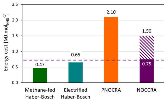
Fig. 3 Energy requirement [MJ mol NH 3 -1 ] of the ammonia synthesis processes: natural gas-based Haber–Bosch, 2 electrified Haber–Bosch, 2 PNOCR 31 and NOCCRA with and without accounting for the savings of NH 3 by avoiding the need for an S(N)CR process for NO x abatement.
