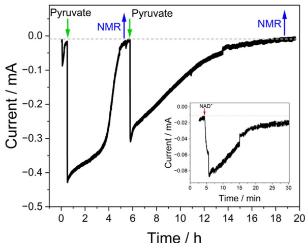
Fig. 6 The synthesis of L-lactate by LDH driven via Y354S. Potential was held at -0.53 V vs. SHE to drive the reduction. The reaction solution was pre-purged with argon and the headspace was continuously purged throughout to remove the contribution to the current from oxygen. All additions of \text{NAD}^+ ( 50\text{ }\mu\text{M} ) and pyruvate (separate 5\text{ mM} additions) were in real-time, as was the removal of samples for NMR analysis. The inset shows a magnification of the addition of \text{NAD}^+ at the start of the experiment. Experiment conditions: buffer: 50\text{ mM} MES, 50\text{ mM} TAPS pH 9; voltage held at -0.53 V vs. SHE; electrode Y354S + LDH@ITO/Ti foil (4 electrode booklet); cell solution purged with argon to remove the contribution to the current from oxygen. Enzymes were loaded into the porous electrode from dilute solution; see Experimental for amounts.
