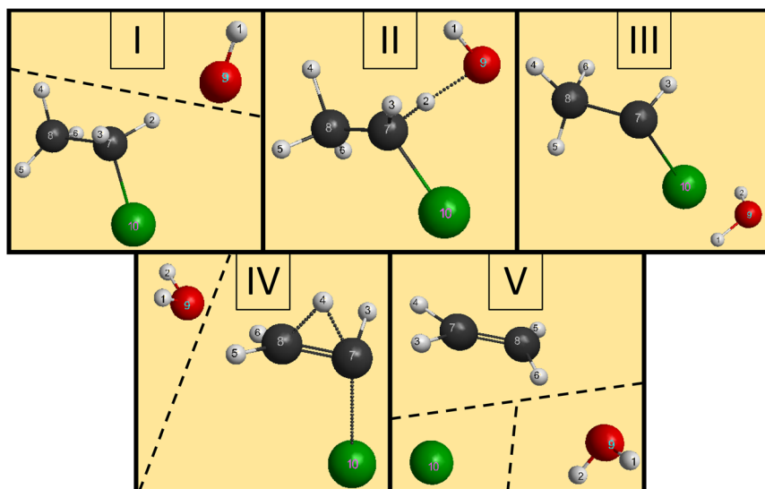
Fig. 5 The main steps of the E2 reaction in the \text{OH}^- + \text{CH}_3\text{CH}_2\text{Cl} system with the \beta\text{--}\alpha transfer mechanism. The dashed line means the species are well separated in space. (I) The reactants approach each other. (II) A proton abstraction (H2) occurs from \text{C}_\alpha (C7), forming water. (III) The newly-formed \text{H}_2\text{O} orbits around the remnant fragment. (IV) The water leaves the remnant anion, the \text{C}_\alpha\text{--Cl} (C7–Cl10) bond gets elongated, while a proton (H4) interacts with both of the carbon atoms. (V) The \text{C}_\alpha\text{--Cl} (C7–Cl10) bond breaks, a chloride ion leaves, the original \text{C}_\beta\text{--H} (C8–H4) bond breaks, while a new \text{C}_\alpha\text{--H} (C7–H4) bond is formed, leading to ethylene.
