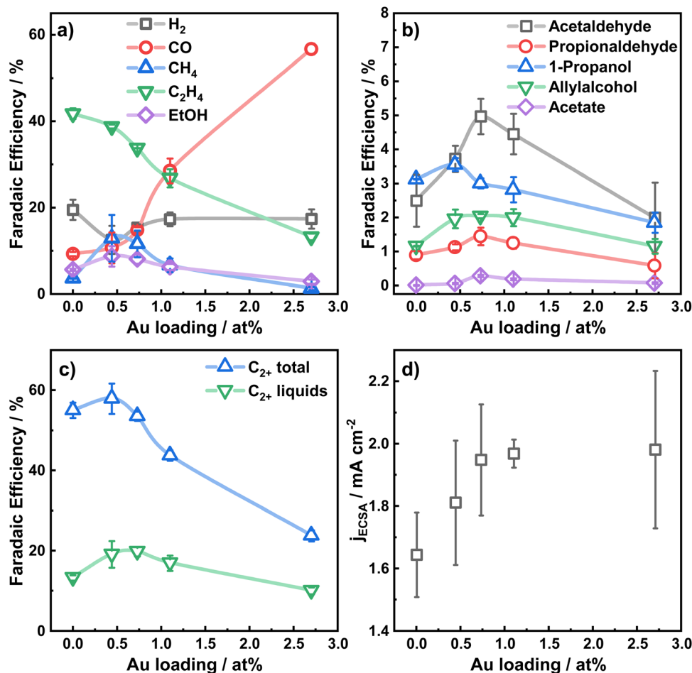
Fig. 2 Faradaic efficiencies at -1.07 V in 0.1 M \text{KHCO}_3 as a function of the Au NP loading for (a) \text{H}_2 , \text{CO} , \text{CH}_4 , \text{C}_2\text{H}_4 , (b) minor liquid products, (c) \text{C}_{2+} total products, \text{C}_{2+} liquid products; (d) Au-loading dependency of the current density normalized by the electrochemical surface area.
