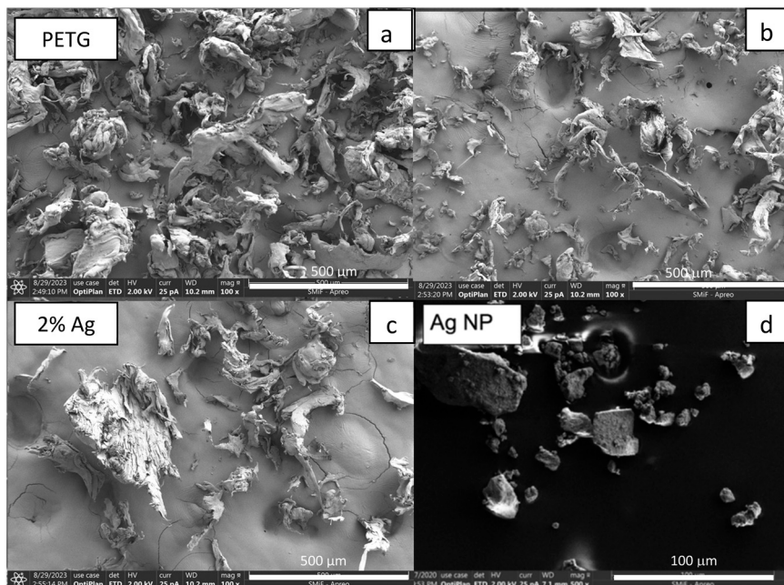
Fig. 4 SEM micrographs of a) PETG, b) 0.5%Aq, c) 2%Aq, and d) Aq nanoparticles. Note the scale bar ranges from 100 \mu\text{m} to 1 mm.
