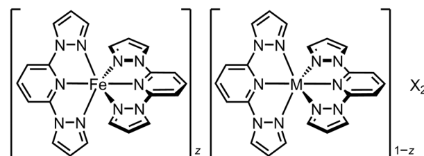
Scheme 1 The solid solutions [\text{Fe}_2\text{M}_{1-z}(1\text{-bpp})_2][\text{BF}_4]_2 (1-bpp = 2,6-bis{pyrazol-1-yl}pyridine; \text{M}^{2+} = \text{Co}^{2+} , \text{Ni}^{2+} , \text{Zn}^{2+} or \text{Ru}^{2+} ; \text{X}^- = \text{BF}_4^- or \text{ClO}_4^- ). 63
