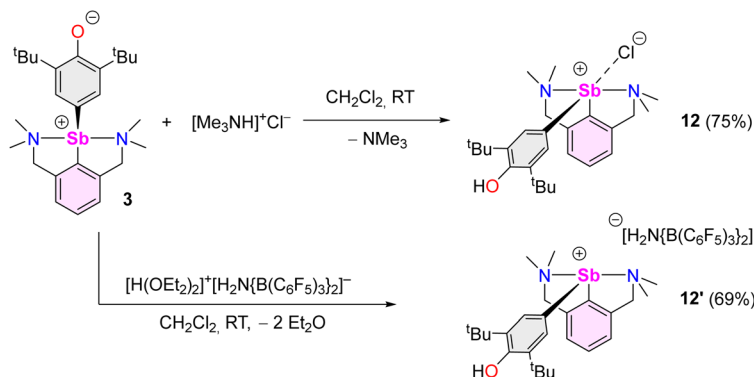
Scheme 4 Synthesis of [\{\text{NCN}^{\text{Me}_4}\}\text{Sb}(\text{C}_6\text{H}_2\text{-}^t\text{Bu}_2\text{-}3,5\text{-OH-}4)][\text{X}] ( \text{X} = \text{Cl} , 12 ; \text{H}_2\text{N}(\text{B}(\text{C}_6\text{F}_5)_3)_2 , 12' ).
