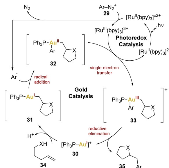
Scheme 7 Proposed mechanism employing a mononuclear gold(I) catalyst and a Ru(II) photococatalyst in a oxy- and aminoarylation of alkenes.
