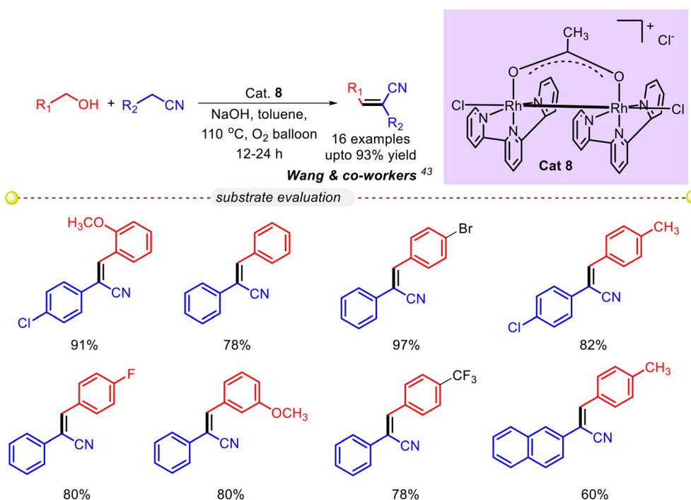
Scheme 14 Rh-binuclear complex catalyzed \alpha -olefination of nitriles using alcohols. 43
