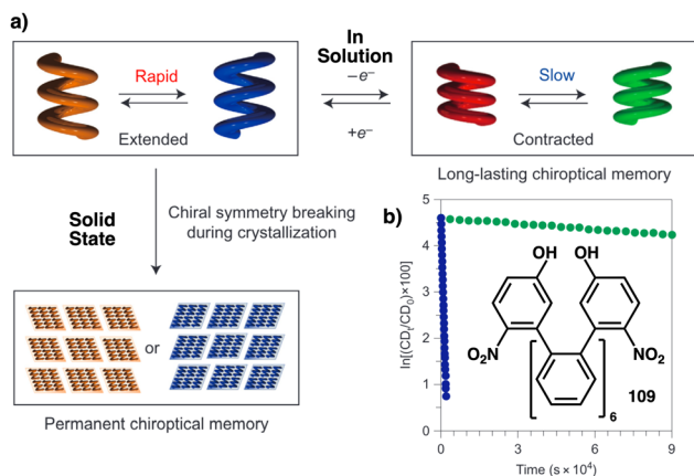
Fig. 51 (a) Schematic representation of the helical inversion dynamics of oligomer 109 in solution and in solid state. (b) chemical structures of 109 and decay profiles of the CD intensities in spectra of the oligomer dissolved in MeCN at 265 nm and the oligomer dissolved in MeCN in the presence of the one-electron oxidant (4-BrC 6 H 4 ) 3 N + [SbCl 6 - ] at 273 nm (green). Reproduced from ref. 251 with permission from Springer Nature, copyright 2010.
