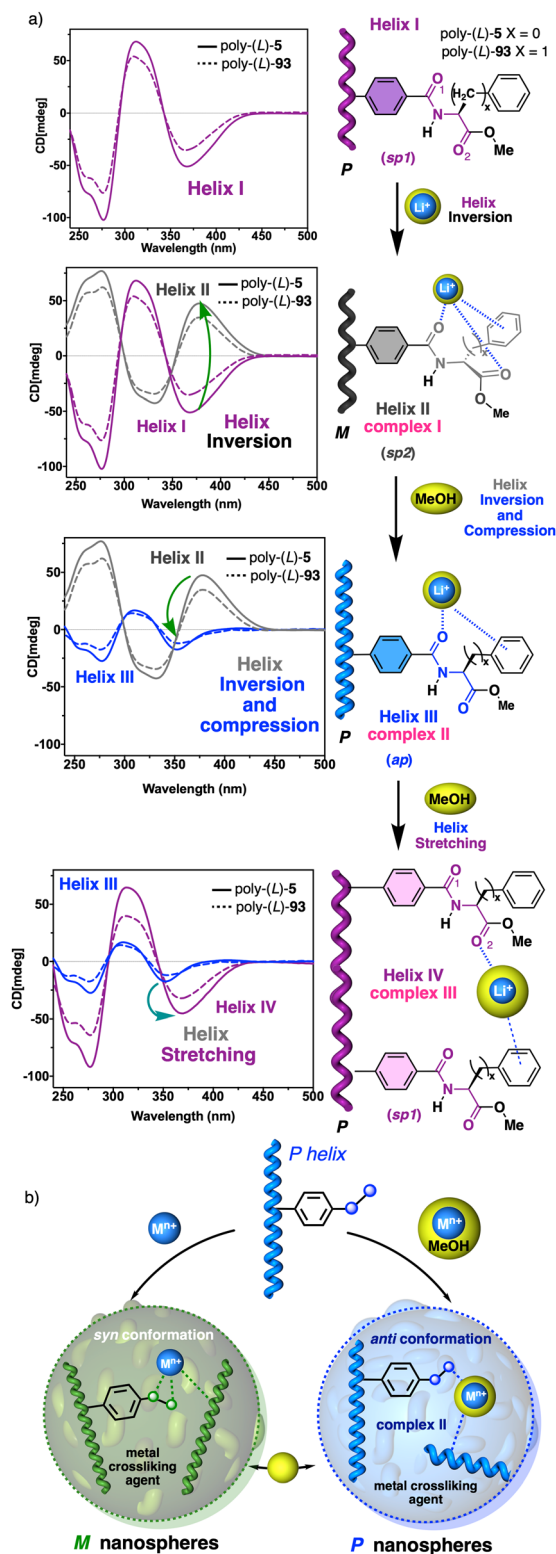
Fig. 40 (a) Elongation and helical sense control via dynamic coordination chemistry in poly-(L)-5 and poly-(L)-93/ \text{Li}^+ /MeOH complexes. (b) Illustration of nanostructuring via dynamic coordination chemistry. Reproduced from ref. 229 with permission from the Royal Society of Chemistry, copyright 2017.
