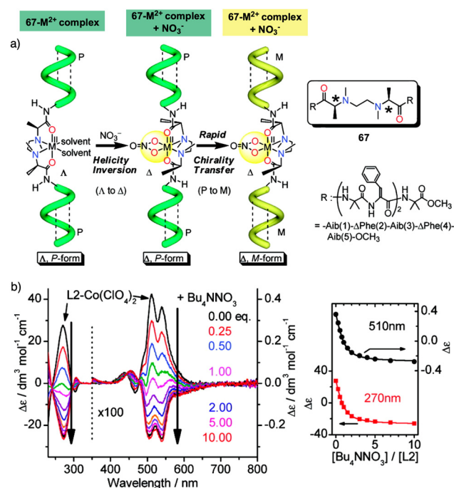
Fig. 19 (a) Anion induced helix inversion of metallo-foldamer 67-M 2+ (M 2+ = Co, Zn, Ni). (b) CD spectra changes of the 67-Co(ClO 4 ) 2 complex upon addition of Bu 4 NNO 3 and titration profiles of the CD wavelength at 270 and 510 nm. Reproduced from ref. 178 with permission from the American Chemical Society, copyright 2008.
