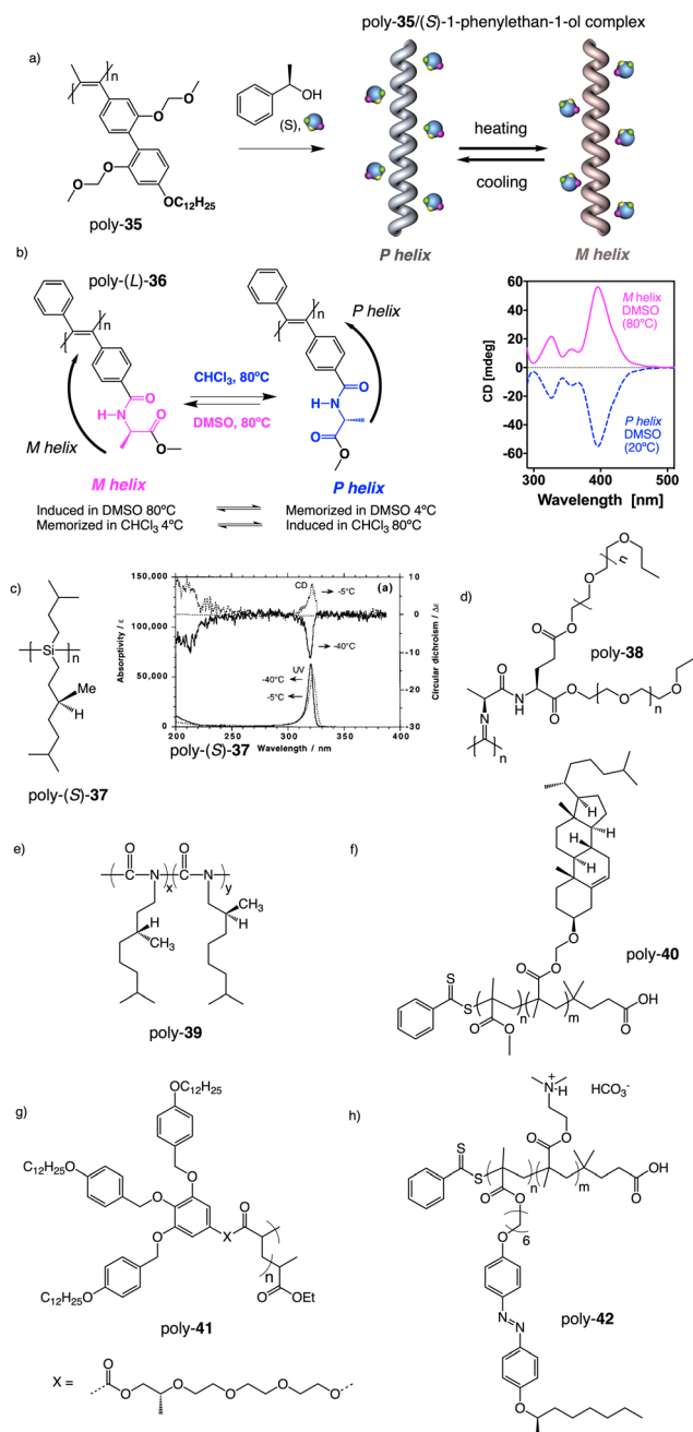
Fig. 11 Thermal driven helix inversion of (a) PBPA poly-35, (b) PDPA poly-36 and (c) polysilylene, poly-37 (reproduced from ref. 149 with permission from the American Chemical Society, copyright 2000). Chemical structures of (d) polyisocyanide poly-38, (e) co-polyisocyanate poly-39, (f) PMMA poly-40, (g) polyacrylate poly-41, (h) PMMA poly-42.
