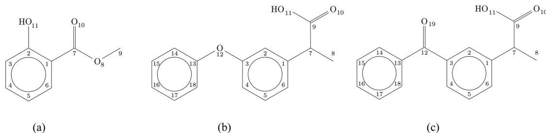
Fig. 1 Schematic structure and numbering of the atoms of (a) methyl salicylate (MS), (b) fenopropfen (FP) and (c) ketopropfen (KP).
