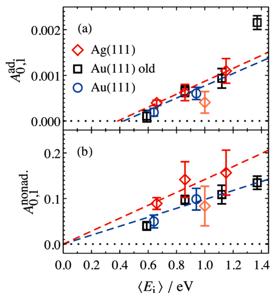
Fig. 4 Decomposition of vibrational excitation for HCl interacting with Au and Ag into adiabatic (a) and nonadiabatic (b) components. A_{0,1}^{nonad}(E_i) extrapolates to zero threshold, while A_{0,1}^{ad}(E_i) extrapolates to 0.39 \pm 0.05 eV and 0.43 \pm 0.19 eV for HCl on Ag(111) and Au(111), respectively. Both thresholds are close to HCl vibrational energy spacing of 0.36 eV. From ref. 57 with permission from American Institute of Physics Copyright (2020).
