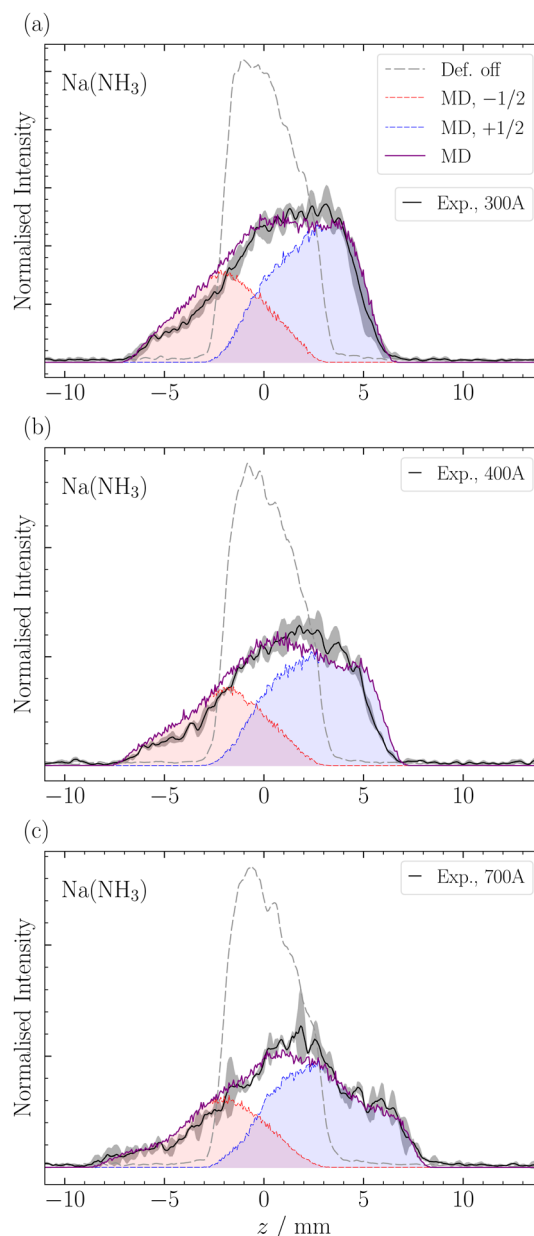
Fig. 4 Magnetic deflection of \text{Na}(\text{NH}_3) measured at a magnification of M_r = 1 and a current of 300 A, 400 A, and 700 A ((a)–(c)). The dashed grey and the black lines correspond to the experimental spatial distribution when the deflector is off and on, respectively. The purple line illustrates the total deflection obtained in our simulations, while the red and blue lines delineate the contributions of the two spin projections. Shaded areas represent experimental uncertainties at 1\sigma .
