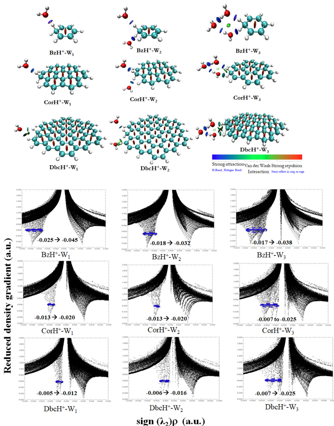
Fig. 3 Top: NCI indexes of the BzH + -W n , CorH + -W n and DbcH + -W n (n = 1–3) clusters with an isosurface of 0.59 a.u. We show the strong and weak interaction regions in blue and green, respectively. Bottom: Bi-dimensional plots of reduced density gradient RDG versus sign(λ 2 )ρ of BzH + -W n , CorH + -W n and DbcH + -W n (n = 1–3) clusters.
