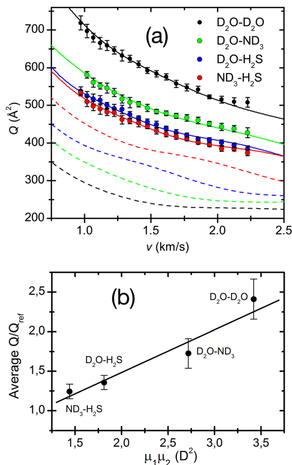
Fig. 8 (a) Total integral collision cross-sections Q(v) , as a function of the collision velocity v , for the D_2O-D_2O , D_2O-ND_3 , D_2O-H_2S and ND_3-H_2S polar pairs. The dashed lines are Q_{ref}(v) calculated for the reference pairs, Ar-Ar (black, reference for D_2O-D_2O ), Ar-Kr (green, reference for D_2O-ND_3 ), Ar-Xe (blue, reference for D_2O-H_2S ) and Kr-Xe (red, reference for ND_3-H_2S ) and convoluted in the laboratory frame under the same conditions. (b) Average ratios of the polar pairs cross-sections versus the reference systems as a function of the permanent dipole product of the polar pairs. 1 D (Debye) = 3.336 \times 10^{-30} C-m. Reproduced from ref. 44 with permission from AIP publishing, copyright © 2014.
