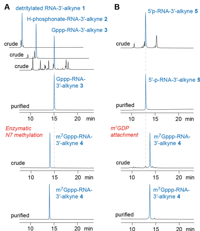
Fig. 3 HPLC analysis of m 7 Gppp-RNA 3'-alkyne preparations (exemplified for m 7 G-5'-ppp-5'-(m 2 Am)(Am)(Cm)(m 3 Um)(3'-O-propargyl-A, RNA 4). (A) Path for chemoenzymatic synthesis. (B) Path for all-chemical synthesis (for details see Fig. 2 and Table 1 and the ESI†).
