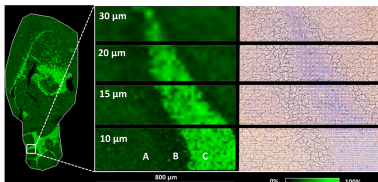
Fig. 3 AgLDI MSI (Ag 6 nm) analysis of cholesterol ( m/z 493.2, [ M + ^{107}\text{Ag} ] ^+ ). The whole brain section (left) at a spatial resolution of 50 \mu m. The mouse cerebellum (middle) at spatial resolutions of 30 \mu m, 20 \mu m, 15 \mu m, and 10 \mu m illustrates the distinct variations in cholesterol intensity between (A) the lobule/molecular layer, (B) the lobule/granular layer, and (C) fiber tracks. An optical microscope image (right) of the mouse cerebellum shows the section after analysis with laser ablation spots.
