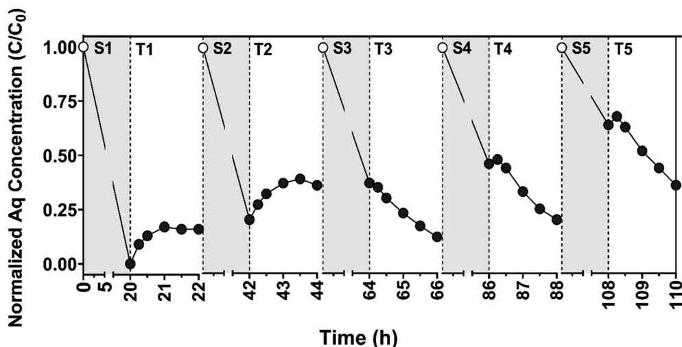
Fig. 7 Normalized aqueous (Aq) CBZ concentration ( C/C_0 ; C_0 = 10 \mu\text{M} CBZ) observed during the sorption (gray) and transformation (white) periods during cycling experiments to test the long-term stability and reactivity of CNF/TiO 2 composites (0.45 g PAN/50 wt% TiO 2 /1000 °C) across five cycles. Electrochemical (EC) transformation occurred at +1.0 V vs. Ag/AgCl. Lines do not represent model fits and are only shown to help illustrate trends in data.
