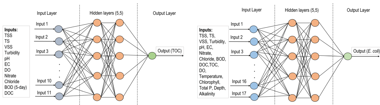
Fig. 2 ANN model architecture for TOC prediction (left) and E. coli prediction (right).
